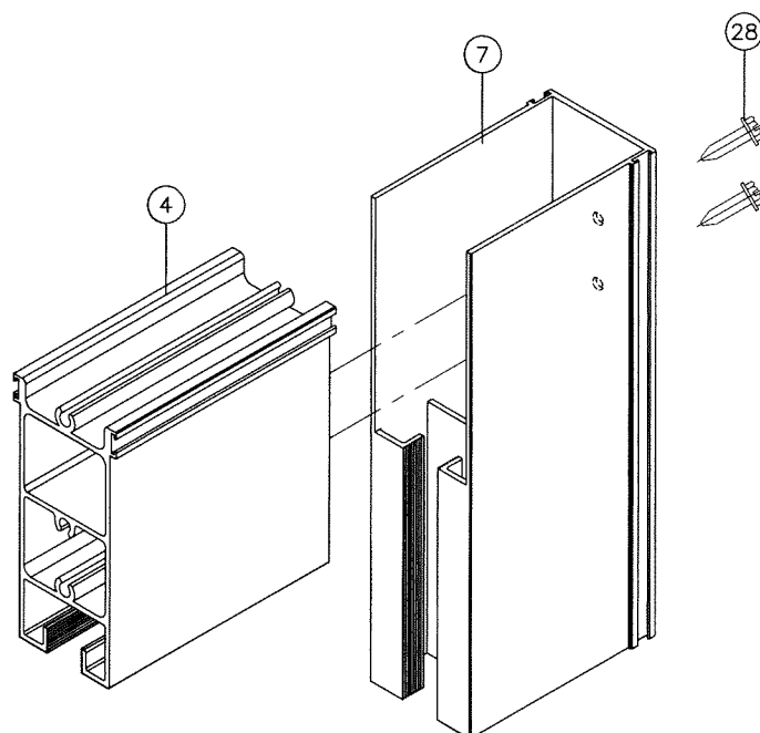
PANEL CORNER
